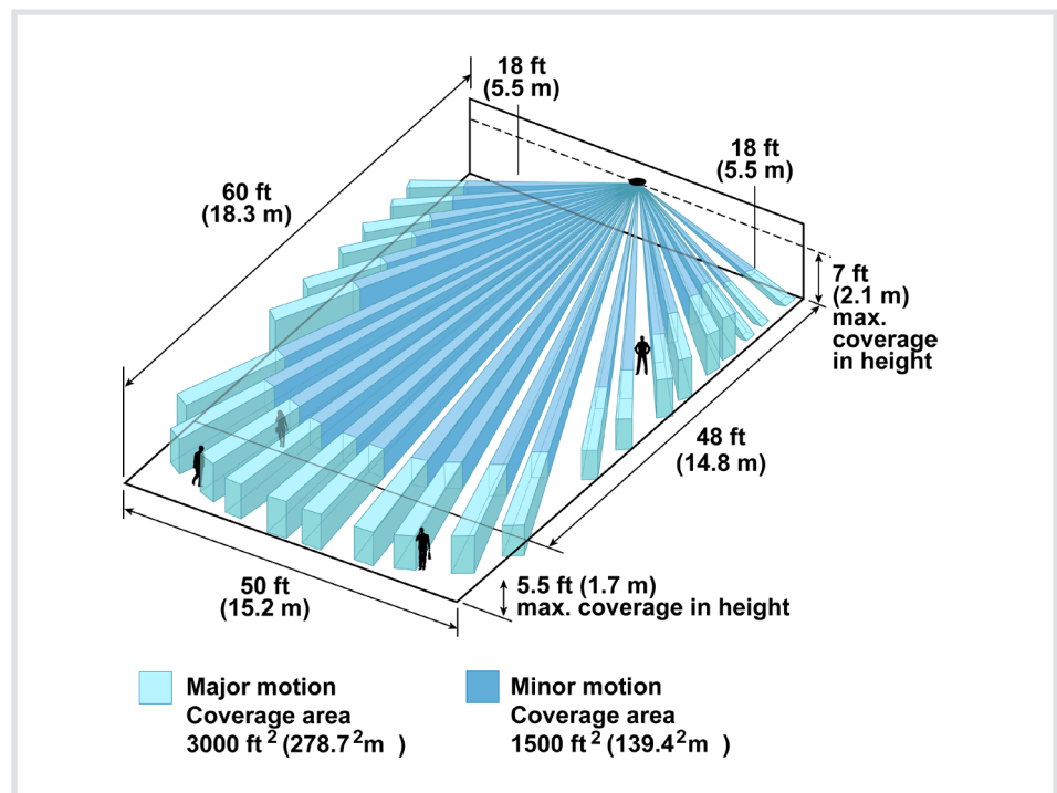
This example shows the detection range for one model of wall-mounted PIR sensors.
