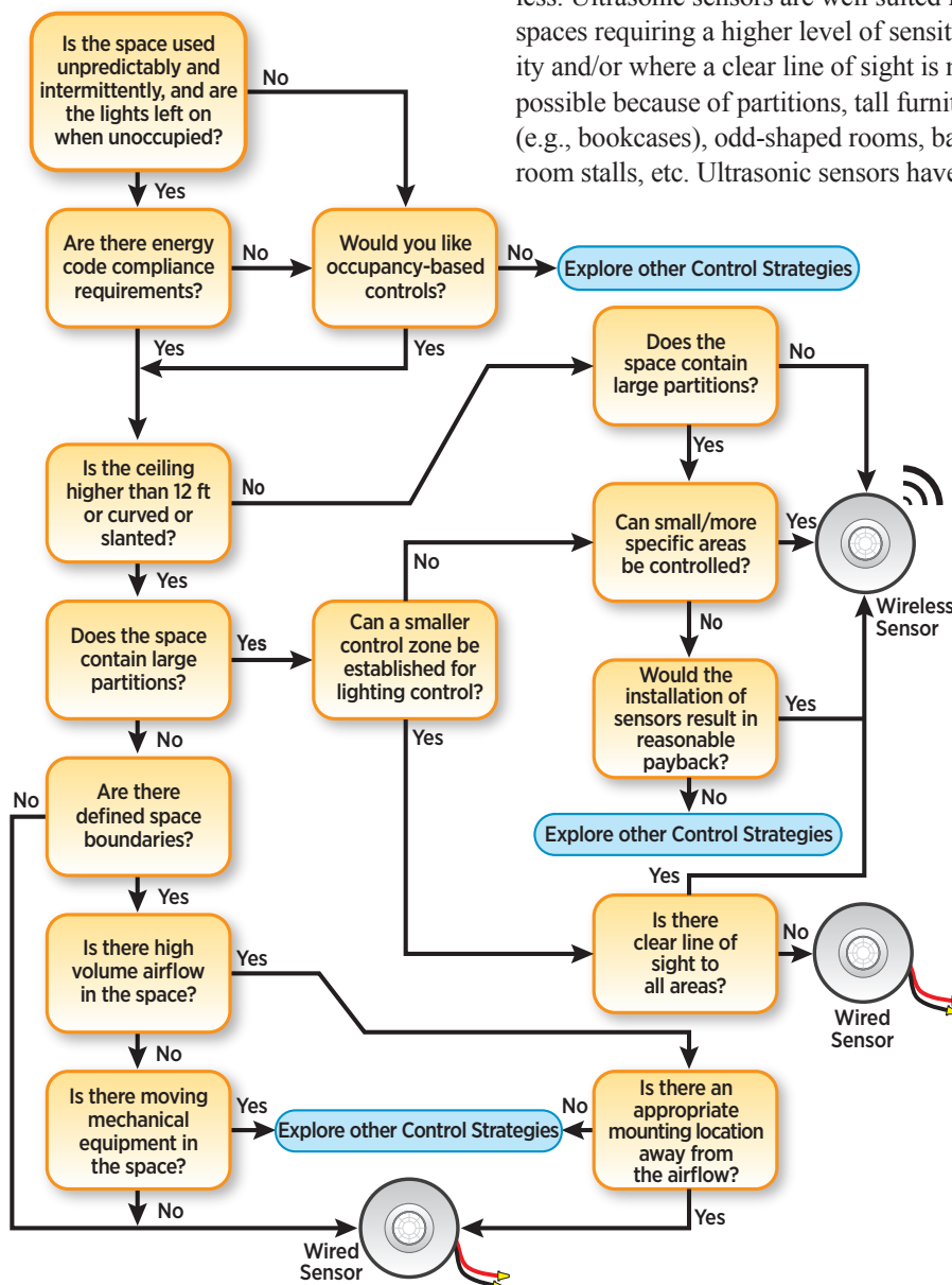
Which Technology Is Best for Your Space? Use this decision tree to determine which lighting control technology is better for a given room - wireless sensors or wired sensors.
