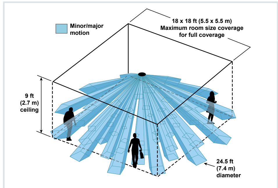
This example shows the detection range for one model of ceiling-mounted PIR sensors.
